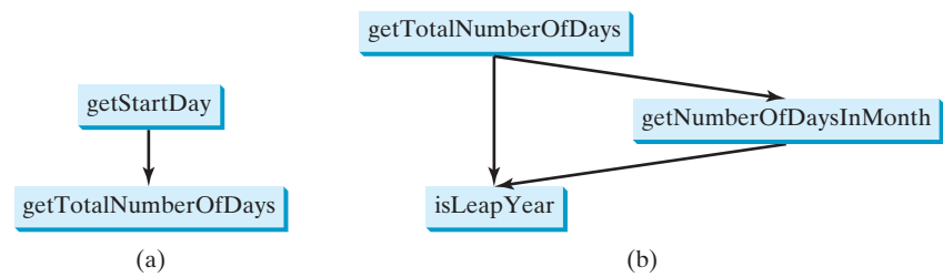
FIGURE 6.13 (a) To accomplish getStartDay , you need getTotalNumberOfDays . (b) The getTotalNumberOfDays problem is refined into two smaller problems.
