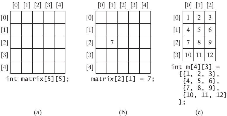
FIGURE 8.1 The index of each subscript of a two-dimensional array is an int value starting from 0 .
