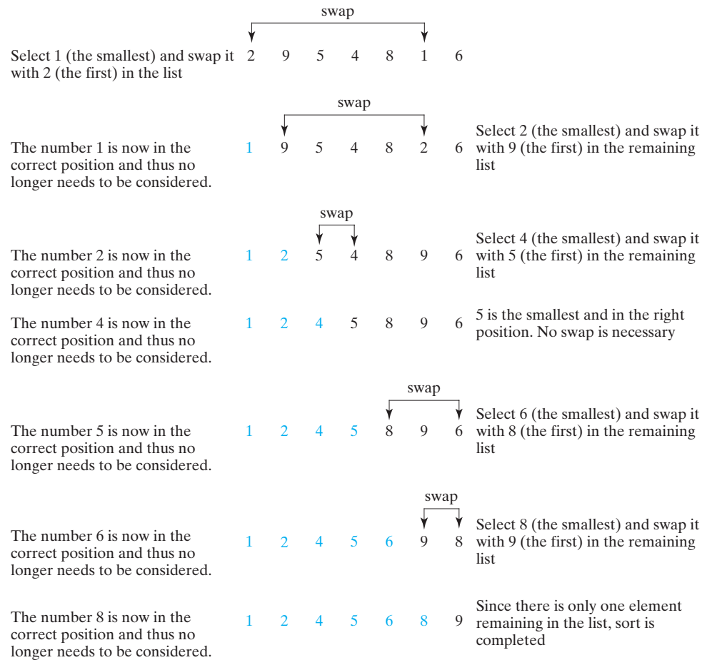
FIGURE 7.8 Selection sort repeatedly selects the smallest number and swaps it with the first number in the remaining list.
