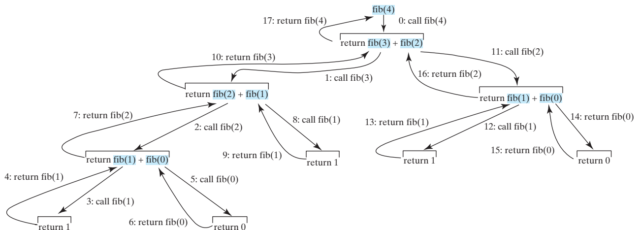
FIGURE 17.4 Invoking fib(4) spawns recursive calls to fib .
