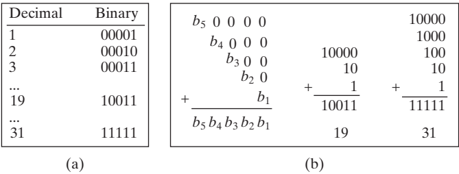
FIGURE 4.1 (a) A number between 1 and 31 can be represented using a 5-digit binary number. (b) A 5-digit binary number can be obtained by adding binary numbers 1, 10, 100, 1000, or 10000.
