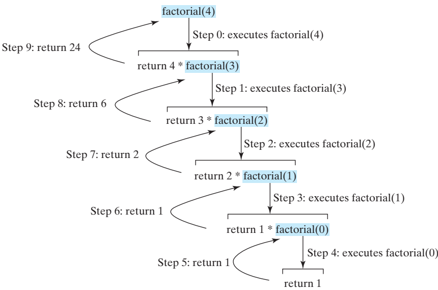
FIGURE 17.2 Invoking factorial(4) spawns recursive calls to factorial .
