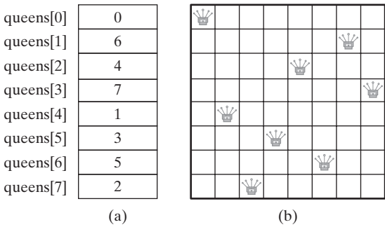
FIGURE 17.8 queens[i] denotes the position of the queen in row i .
