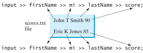
FIGURE 13.2 The input stream reads data from the file.
