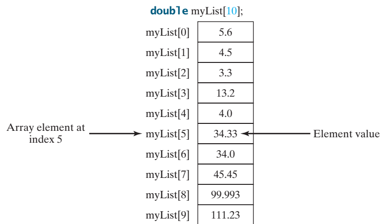
FIGURE 7.1 The array myList has 10 elements of double type and int indices from 0 to 9 .
