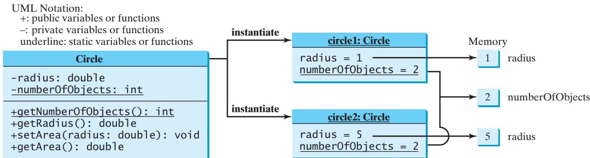
FIGURE 10.10 The instance variables, which belong to the instances, have memory storage independent of one another. The static variables are shared by all the instances of the same class.
