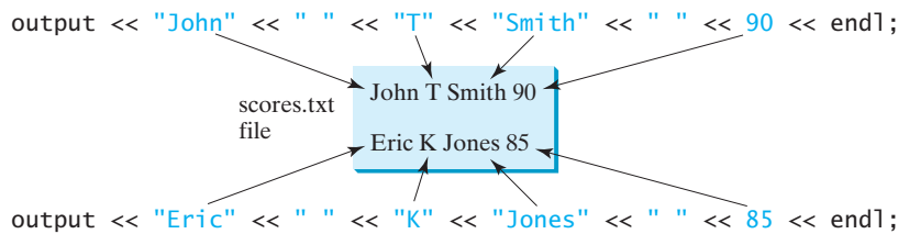
FIGURE 13.1 The output stream sends data to the file.
