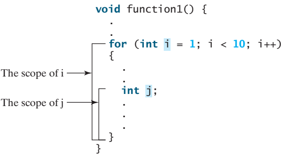
FIGURE 6.4 A variable declared in the initial action part of a for -loop header has its scope in the entire loop.
